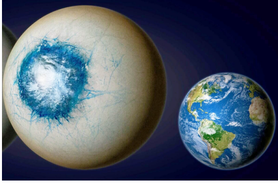
(a) LHS 1140 b ( d_M = 2.779 , 74.3th percentile)
