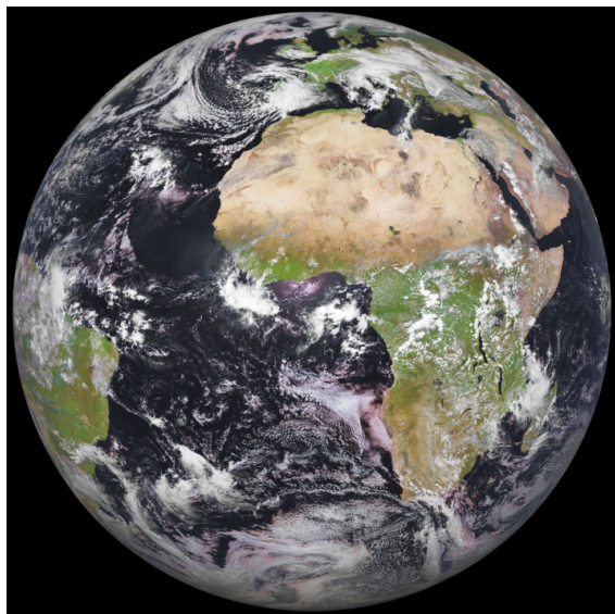
(a) Earth ( d_M = 2.699 , 69.4th percentile)
