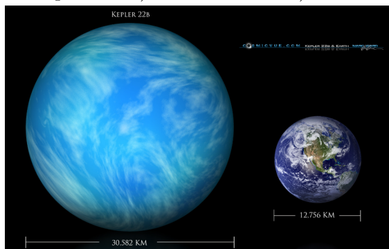
(c) Kepler-22 b ( d_M = 2.728 , 71.2th percentile)
