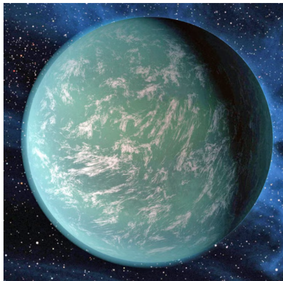
(b) Kepler-22 b ( d_M = 2.728 , 71.2th percentile)
