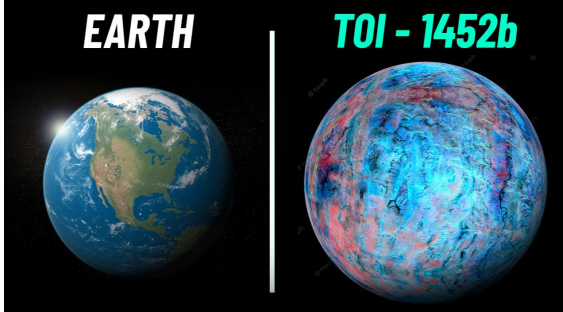
(c) TOI-1452 b ( d_M = 2.384 , 59.2th percentile)
